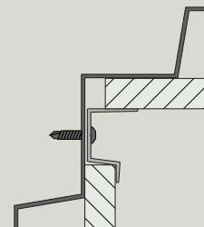
Interior Corner Trim
