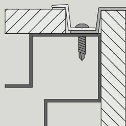
Exterior Corner Trim
